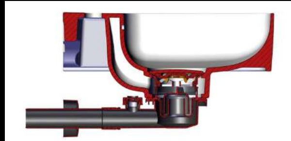
FLAT TRAP SIPHON
